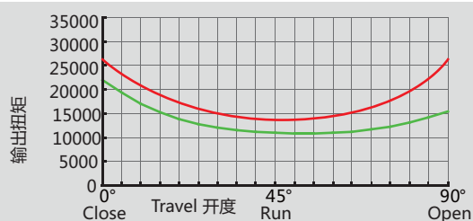
■ 弹簧复位运行曲线 Spring return operating curve
