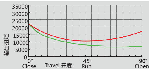
■ 球阀 蝶阀 运行曲线 Ball valve butterfly valve operating curve
